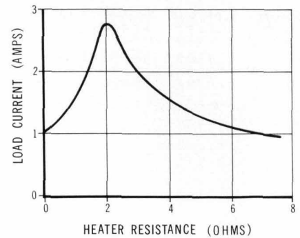
Fig. 4. Maximum current available from klystron heater supply in Model 716A.
