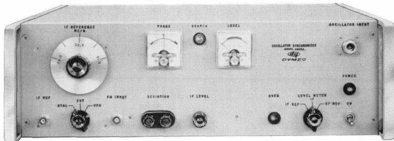
Fig. 3. Dymec DY-2650A Oscillator Synchronizer can be used with most reflex klystrons to achieve high microwave frequency stability. Unit has automatic search and capture capability.
