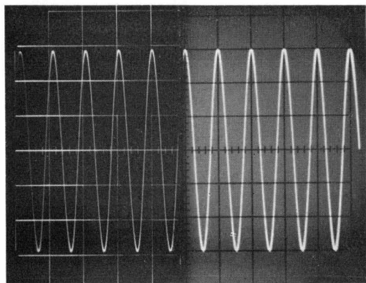
Fig. 2. Oscillogram made on special "half-and-half" showing elimination of parallax error and improved readability of internal-graticule crt.
